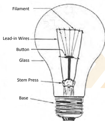
Reference Drawing
